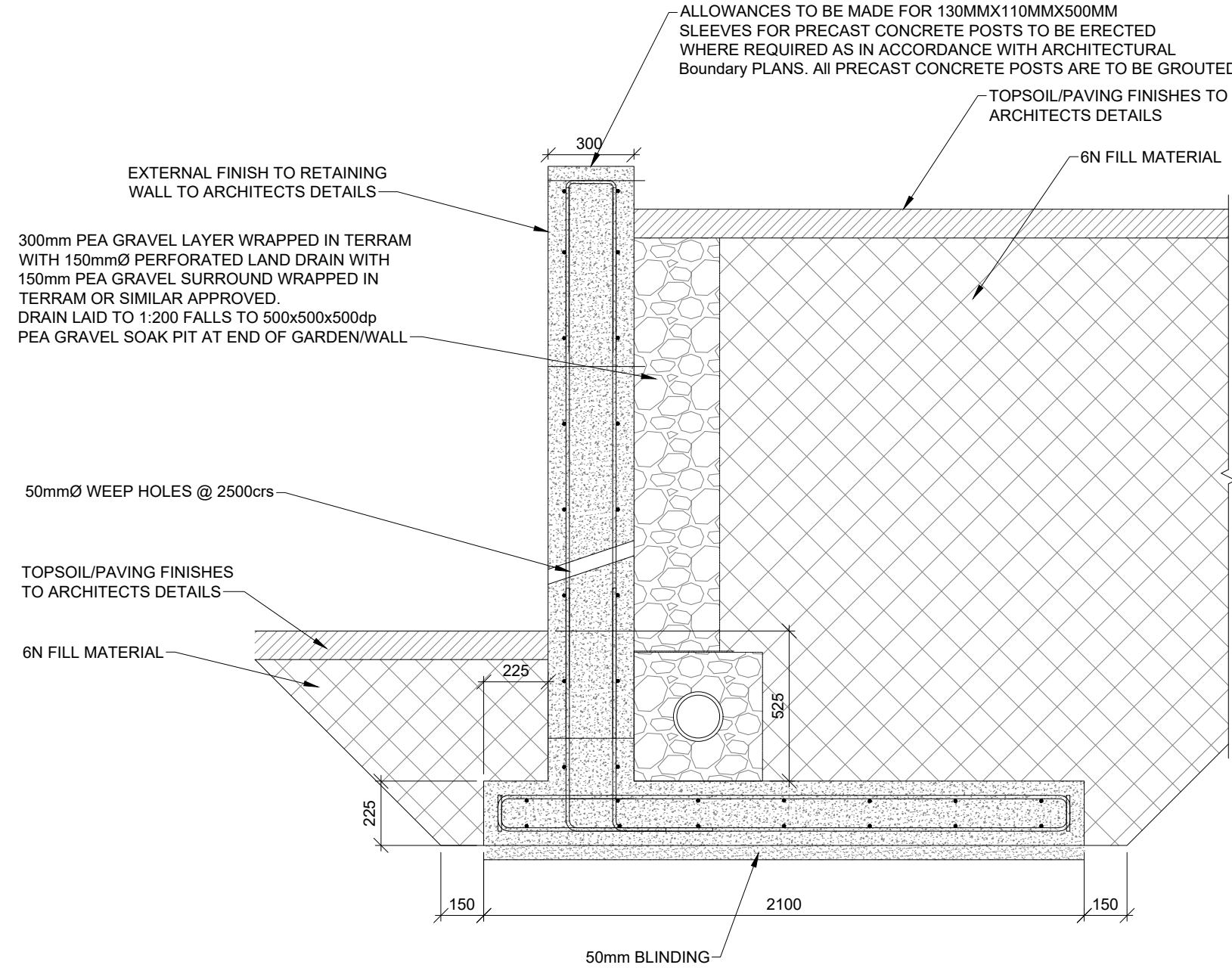
INDICATIVE RETAINING WALL SECTION SCALE 1:20
